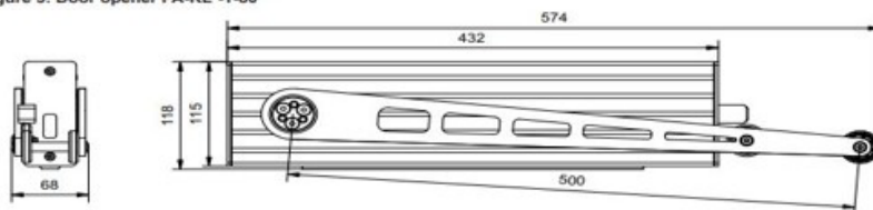
Figure 3: Door opener PA-KL 2 -T-80
