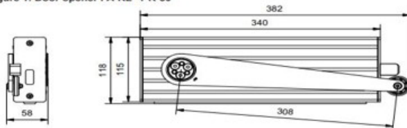
Figure 2: Door opener PA-KL 2 -T-30/PA-KL 2 -T-50
